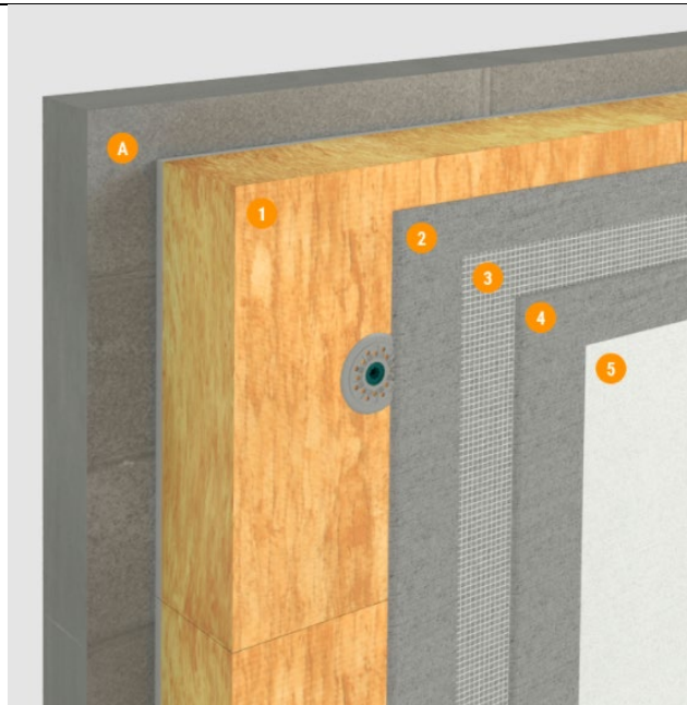
Illustration af Alfix DuraTherm-mineral facadesystem
